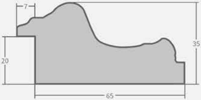
B x H: 72 x 35 mm
